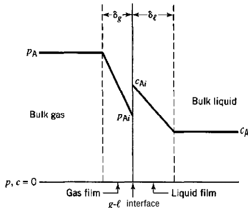
Figure 9.4 Two-film model (profiles) for mass transfer of A from gas phase to liquid phase (no reaction)
