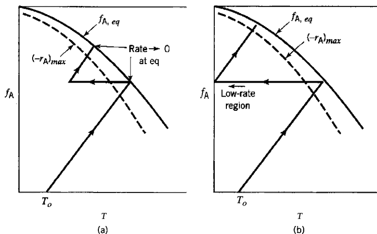
Figure 21.9 Extreme cases for FBCR, both requiring relatively large W(\text{catalyst}) : (a) approach to equilibrium; (b) extent of interstage cooling
