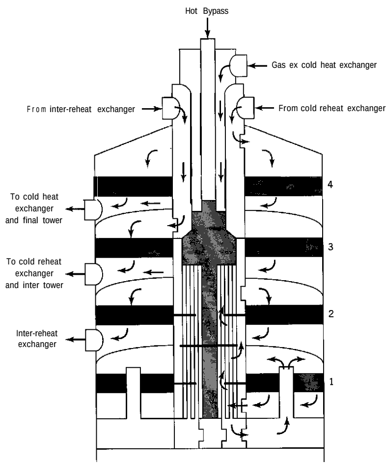
Figure 1.4 Schematic diagram of a four-stage Chemetics SO 2 converter (courtesy Kvaerner-Chemetics Inc.)
