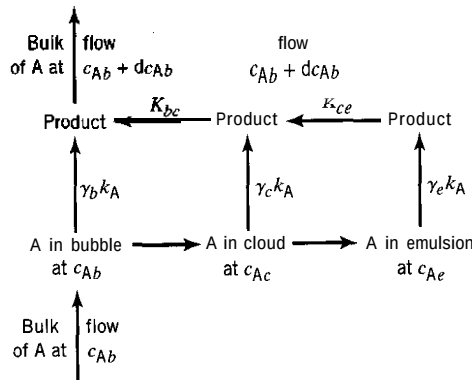
Figure 23.8 Flow/kinetics scheme for bubbling-bed reactor model for reaction A(g) + \dots \rightarrow \text{product(s)}
