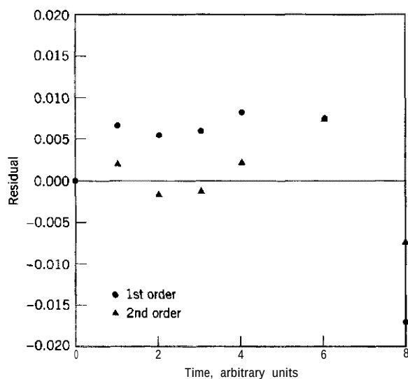
Figure 3.10 Comparison of residual values, c_{A,calc} - c_{A,exp} for first- and second-order fits of data in Example 3-8
