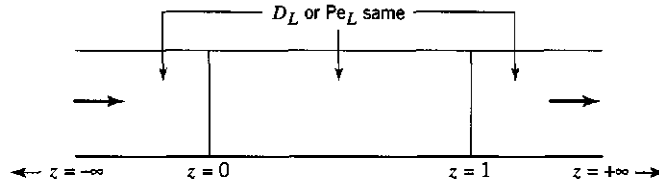
Figure 19.17 Flow conditions for open-open vessel
