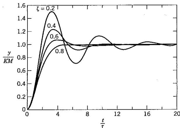
Figure 5.8 Step response of underdamped second-order processes.
