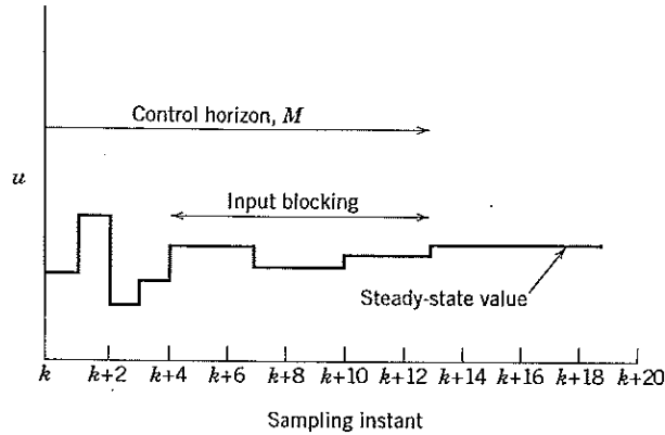
Figure 20.10 Input blocking.
