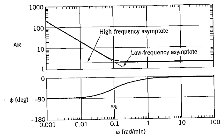
Figure 13.9 Bode plot of a PI controller, G_c(s) = 2 \left( \frac{10s + 1}{10s} \right) .
