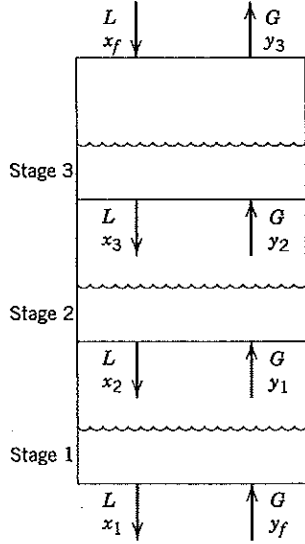
Figure 2.8 A three-stage absorption unit.
