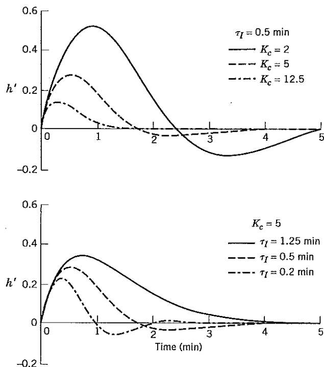
Figure 11.21 Effect of controller settings on disturbance responses ( \tau = 5 min, K_p = 6.37 , K_m = 24 , K_v = 1/60 ).
