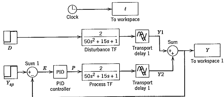
Figure C.4 Closed-loop diagram.
