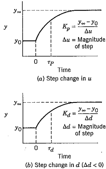
Figure 15.15 The open-loop responses to step changes in u and d .
