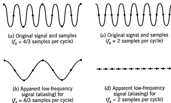
Figure 17.4 Aliasing error due to sampling too slowly.
