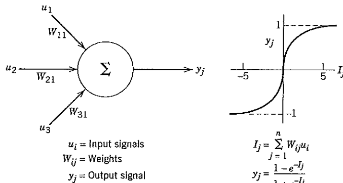
Figure 7.13 Signal diagram for a neuron.
