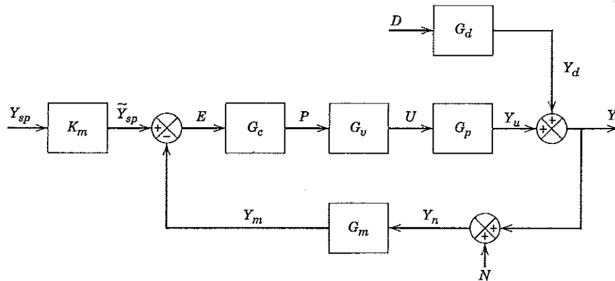
Figure 14.1 Block diagram with a disturbance D and measurement noise N .
