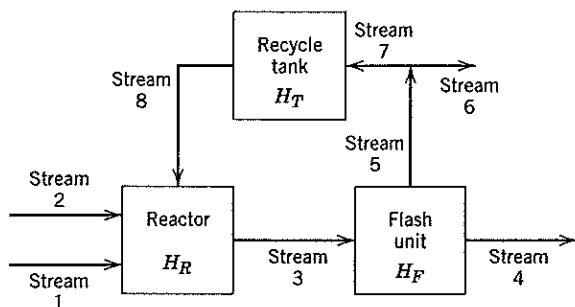
Figure 24.5 Process flow diagram for the core model of the plant: the core model consists of reactor, flash unit, and recycle tank, all operated isothermally and isobarically.
