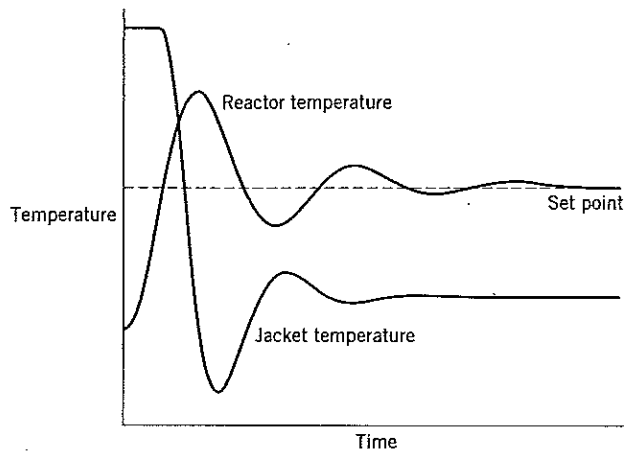
Figure 22.14 Start-up of a batch reactor and the effect of reset windup.
