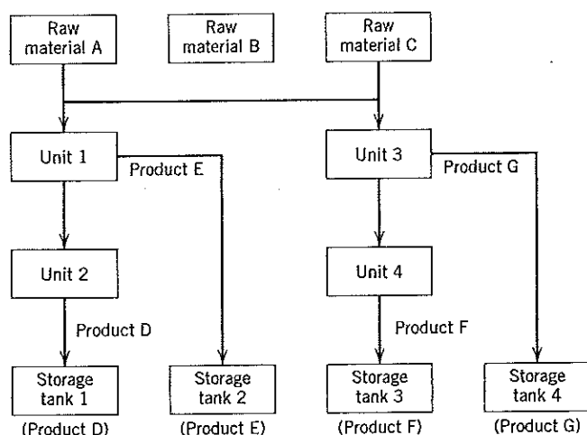
Figure 22.18 Flowsheet for a multiproduct batch plant.
