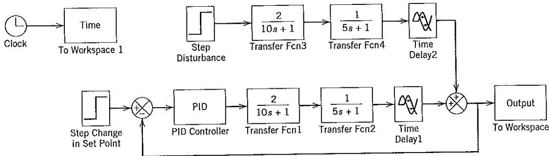
Figure 12.5 Simulink diagram for Example 12.1.
