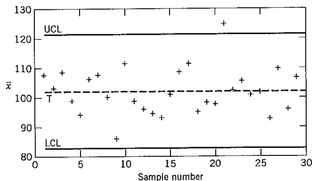
Figure 21.4 The \bar{x} control chart for Example 21.1.
