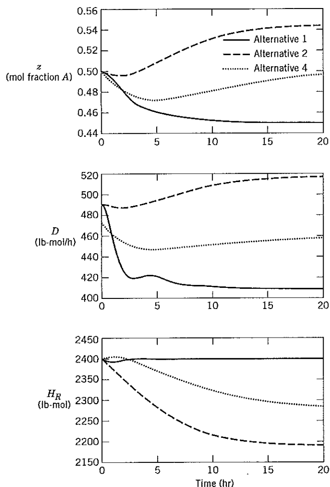
Figure 23.9a Disturbance response of the reactor/distillation column plant using three alternative flow/level control structures ( \sim 10\% change in F_0 ).
