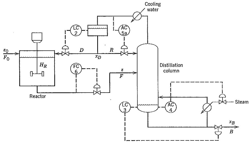
Figure 23.7b Alternative control structures for the reactor/distillation column plant.
