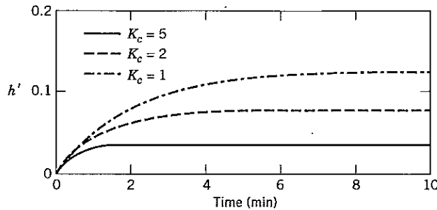
Figure 11.19 Disturbance responses for Example 11.3.
