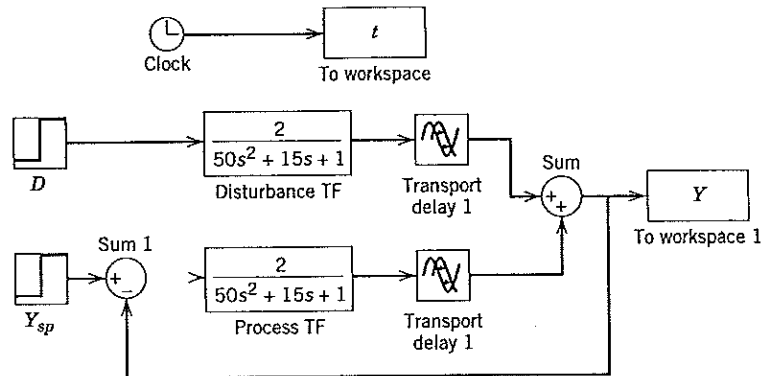
Figure C.3 Partially completed closed-loop diagram.
