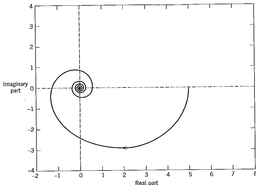
Figure 13.13 The Nyquist diagram for the transfer function in Example 13.5.
