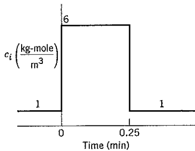
Figure 3.5 Proposed input pulse in reactant concentration.
