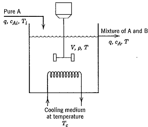
Figure 2.6 A nonisothermal continuous stirred-tank reactor.
