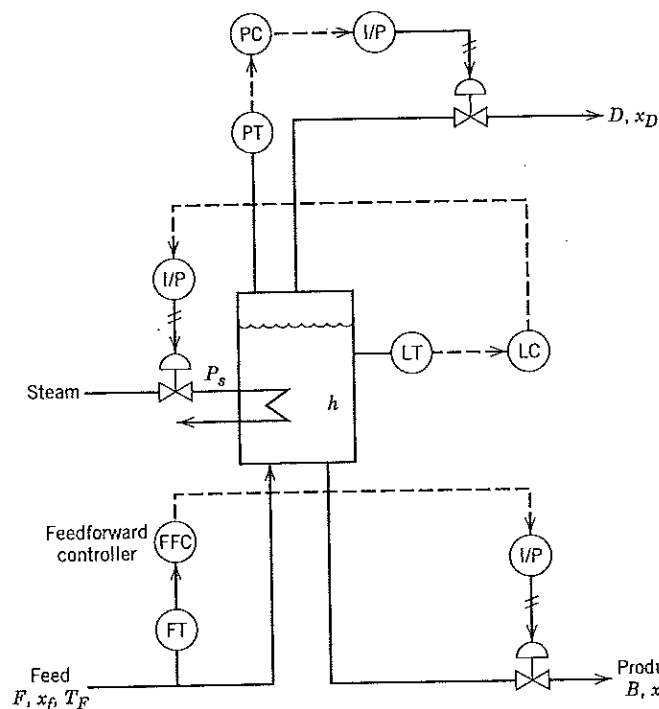
Figure 10.10 Evaporator control strategy for Case (b).
