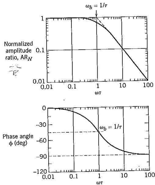
Figure 13.2 Bode diagram for a first-order process.
