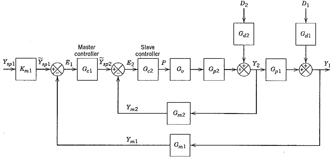
Figure 16.4 Block diagram of the cascade control system.
